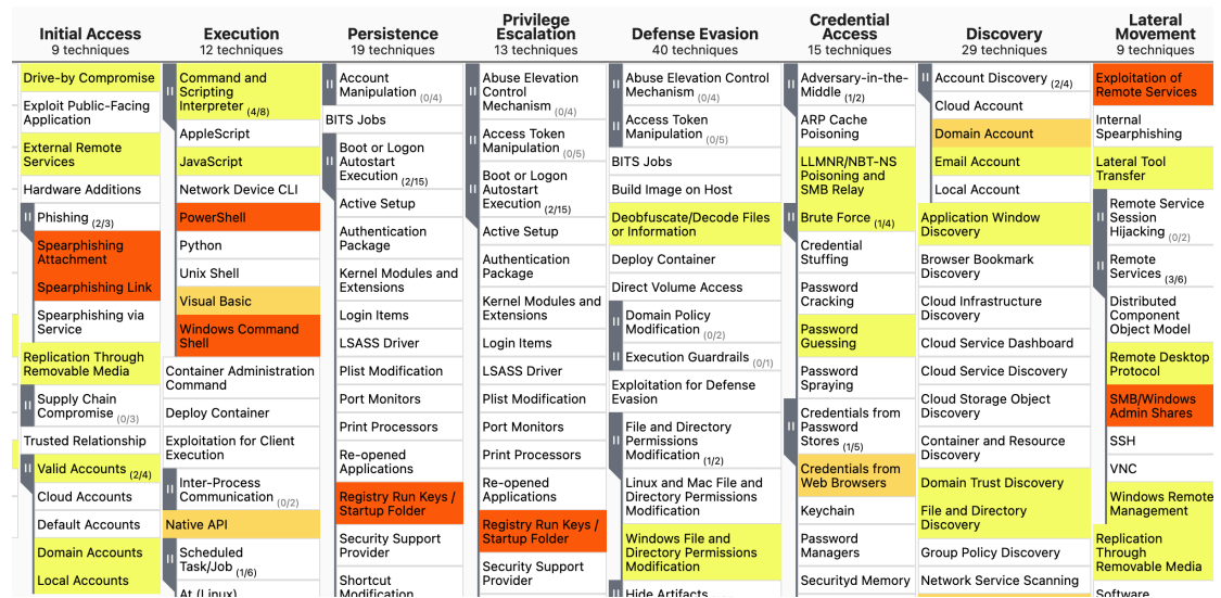
Figure 10 Example of the use of a heatmap to show prevalence of techniques
